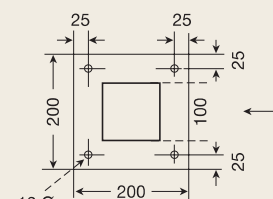
Pivot post
